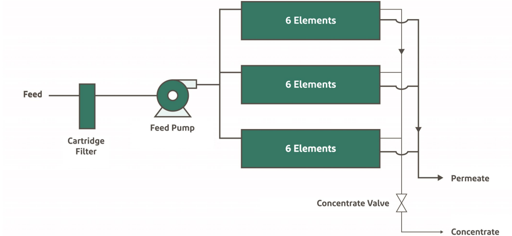
Figure 32. Single-stage system
