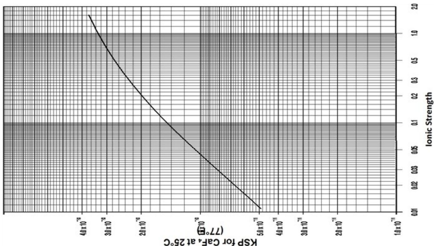
Figure 24. K_{sp} for \text{CaF}_2 versus ionic strength / 11/
