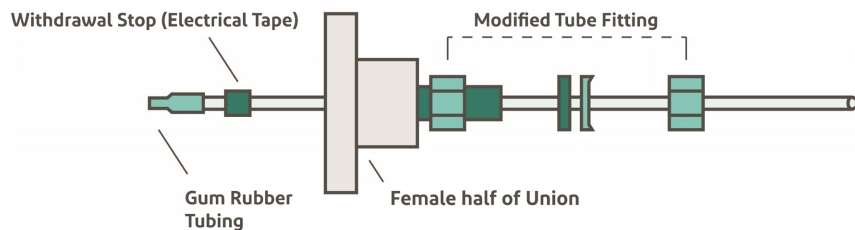
Figure 52. Permeate probing apparatus for spiral-wound membrane
