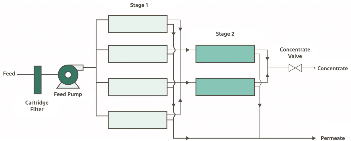
Figure 33. Two-stage system
