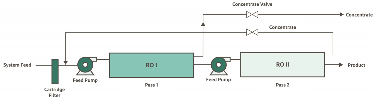
Figure 37. Permeate-staged system
