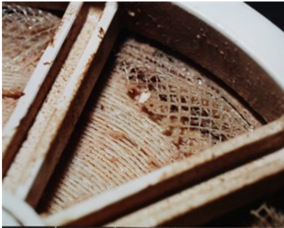
Figure 60. High pressure drop due to biofouling has pushed out the feed spacer
