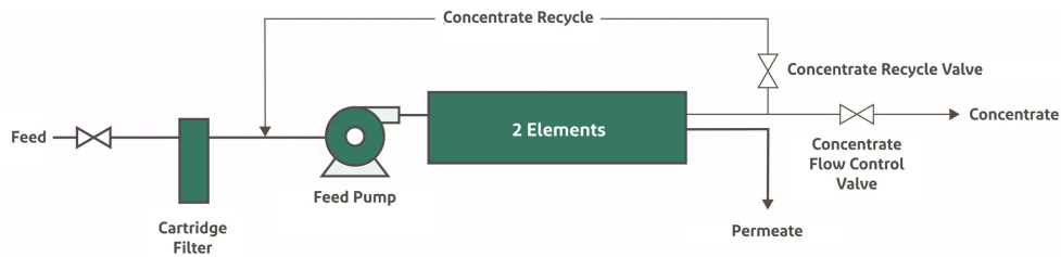
Figure 31. Single-module system
